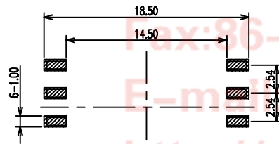
P.C.B HOLE LAYOUT TOP VIEW
