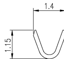
B-B SECTION
