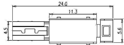
FRONT SHELL
