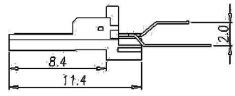
HOUSING + PIN
