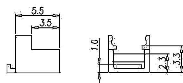
BACK COVER
